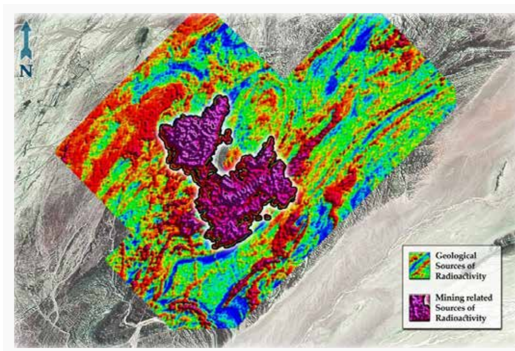
Figure 12: Sources of radioactivity in the mining area
