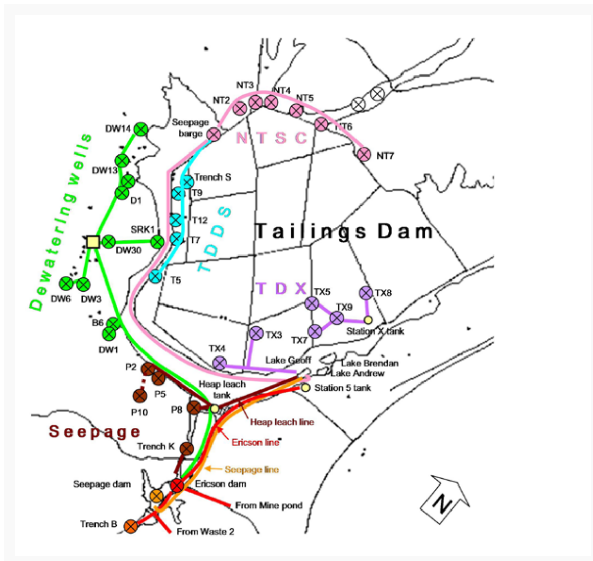
Figure 45: Seepage recovery systems, with de-watering wells (green), tailings dam seepage system (TDDS, blue), northern tailings seepage control (NTSC, pink), tailings dam extraction (TDX, purple) and seepage recovery, brown.
