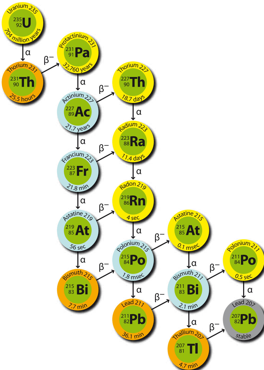
Figure 50: U-235 principal decay modes, with permission from VO Consulting, www.voconsulting.net
