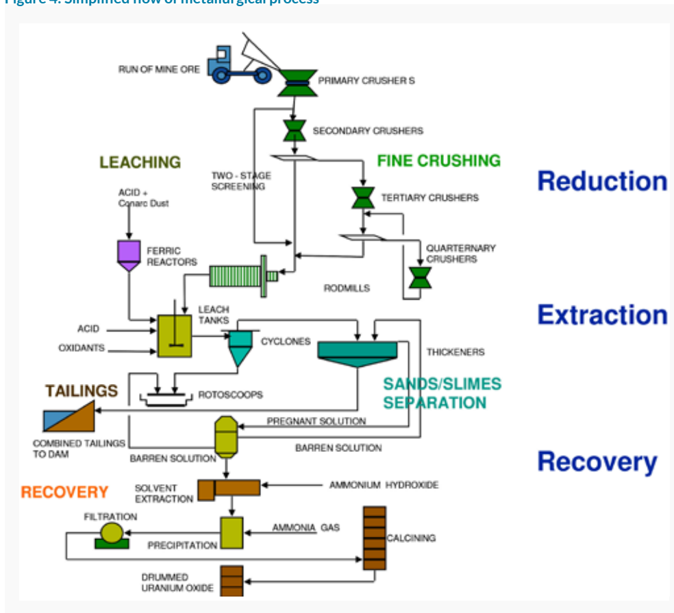
Figure 4: Simplified flow of metallurgical process
