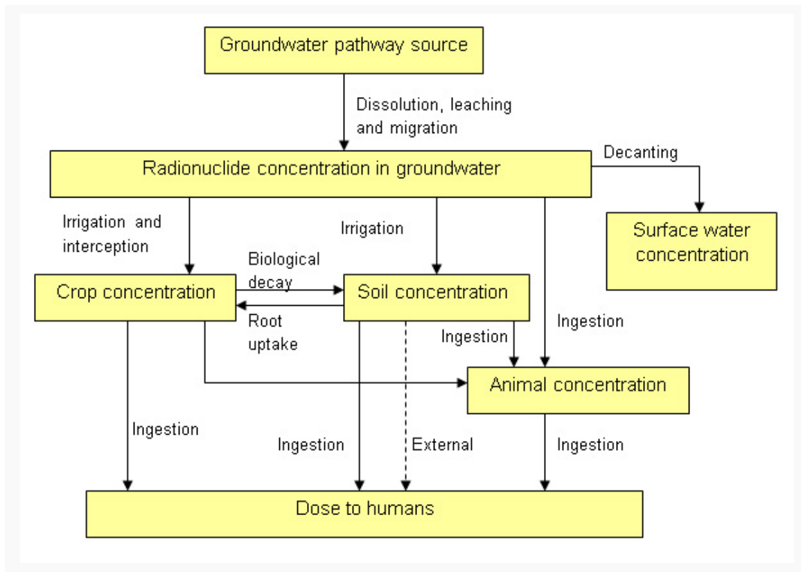
Figure 26: Schematic representation of the pathways and processes associated with the uptake of radionuclides from groundwater.
