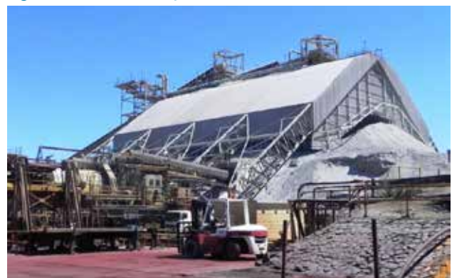
Figure 19: Fine ore stockpile
