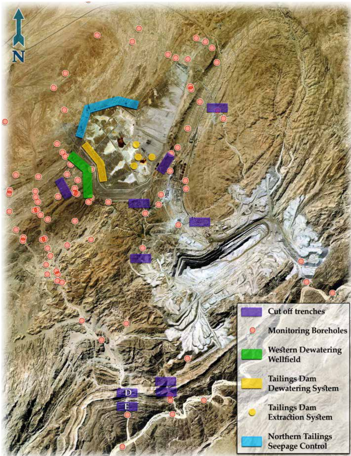
Figure 29: Location of monitoring boreholes at the Rössing mine site
