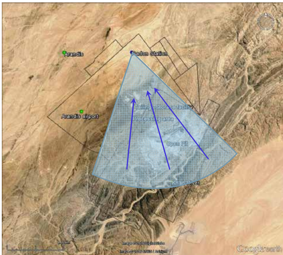
Figure 32: Satellite image displaying Rössing Uranium mine site, radon monitoring station at Arandis, and Arandis town. The wedge indicates the direction from the mine site towards the radon monitoring station, including wind directions which may result in radon concentrations above background at the station.
