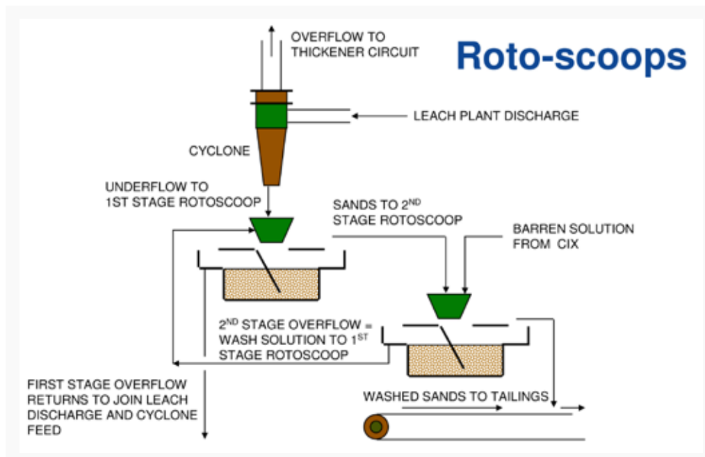
Figure 7: Washing circuits
