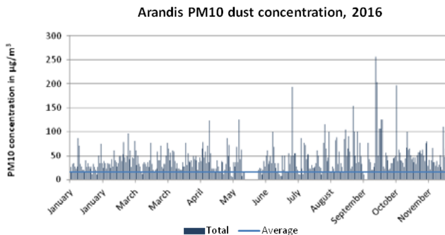
Figure 39: PM10 dust concentration measured in Arandis in intervals of 15 minutes, 2016.
