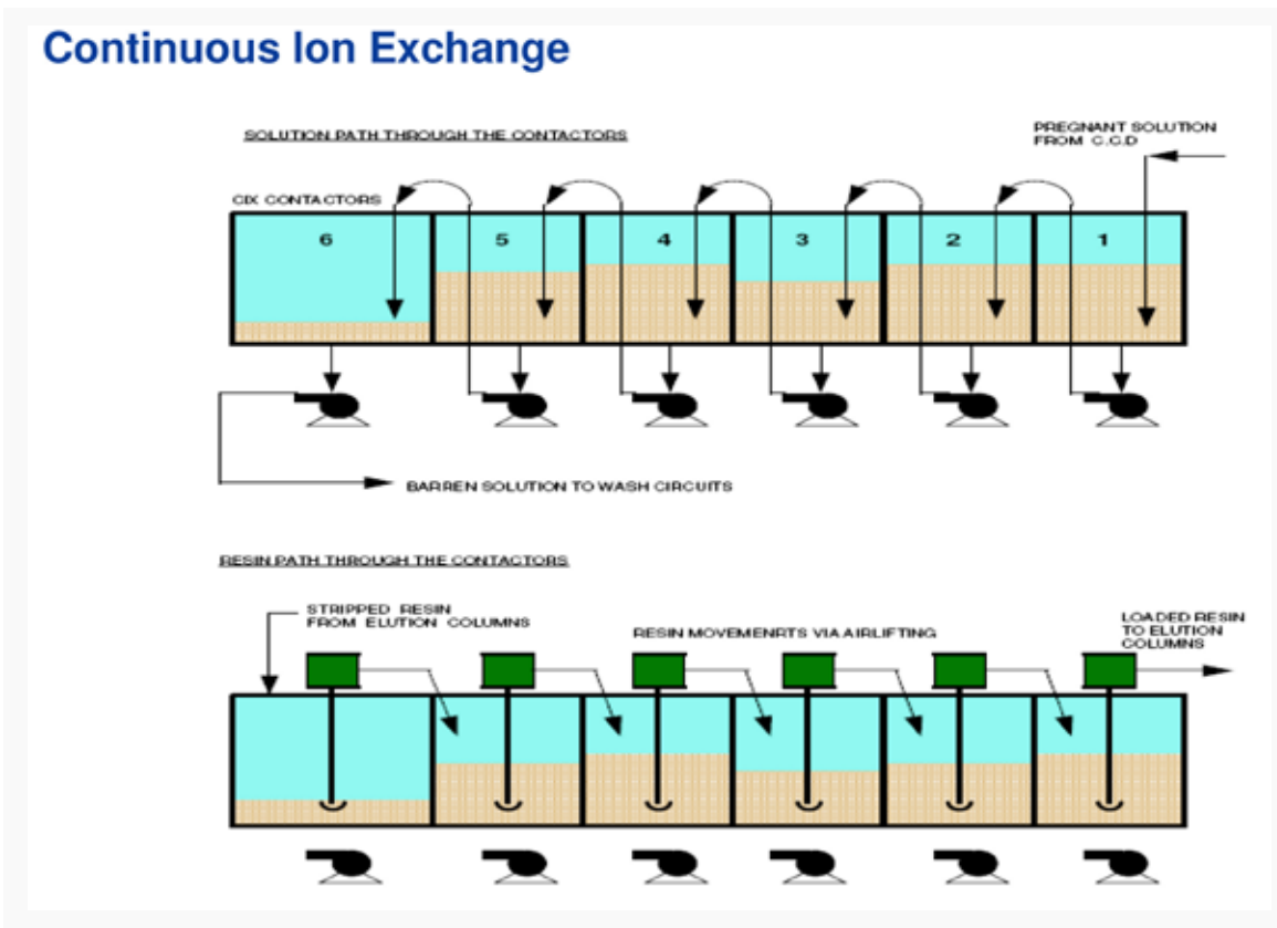
Figure 9: Continuous ion exchange
