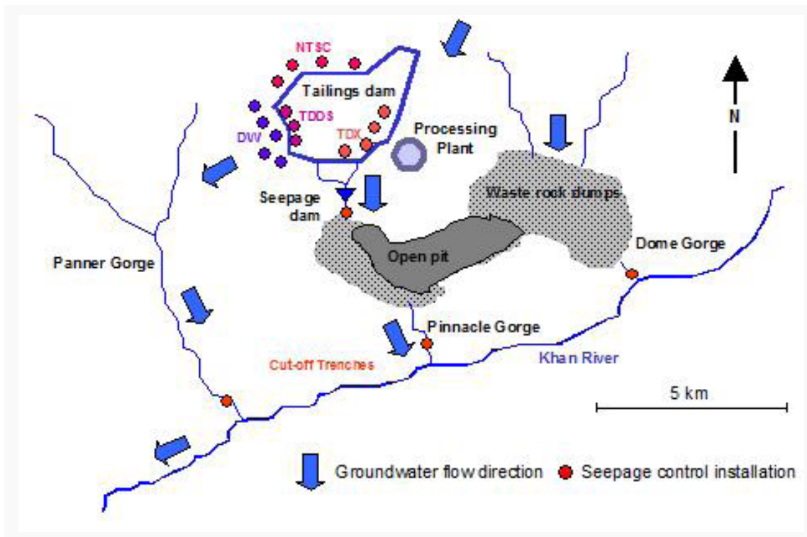
Figure 44: Seepage flow directions and control measures
