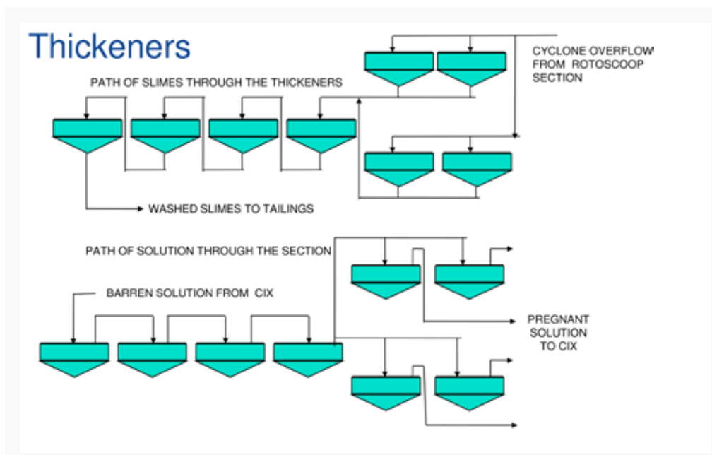
Figure 8: CCD Thickeners
