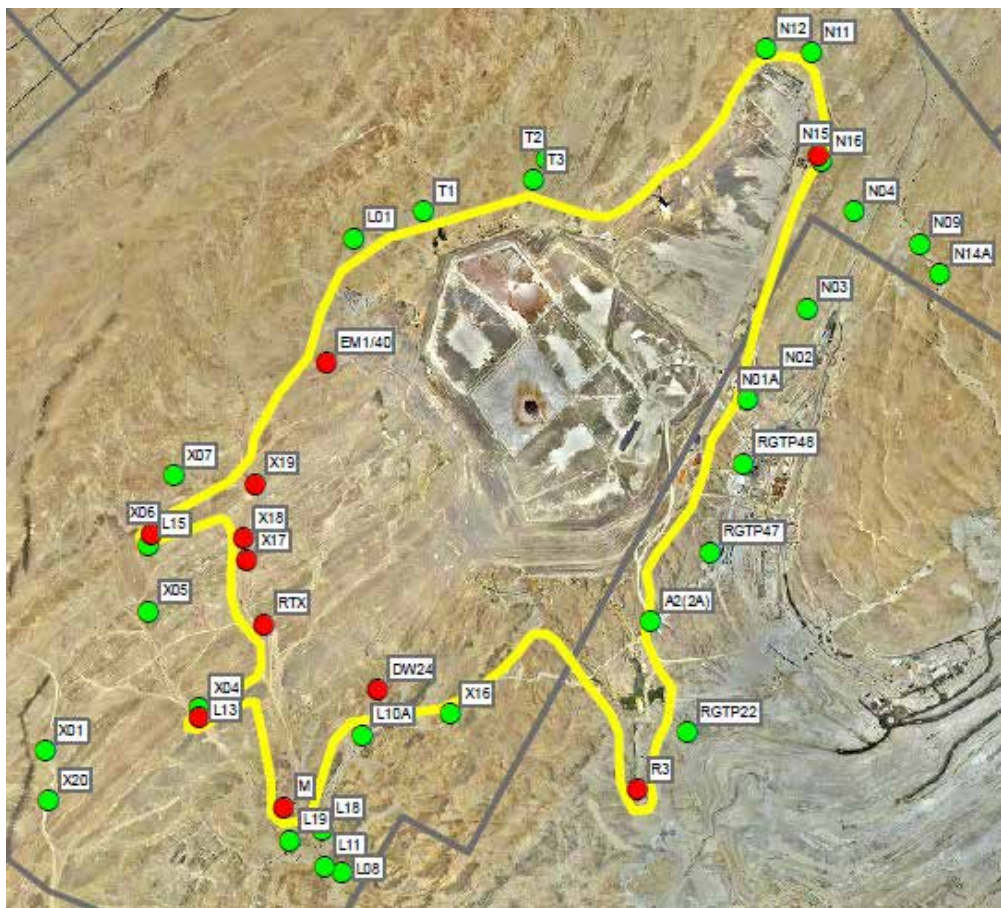
Figure 30: Delineation of the seepage plume surrounding the tailings storage facility (yellow line). Affected bores close to the seepage front are indicated with red circles; unaffected bores with green circles.
