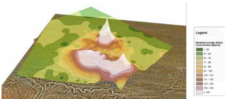
Figure 31: Three-dimensional image of radon concentration overlaying a map of the Rössing Uranium site. The broader peak is on top of the open pit and waste dumps, while the steepest peak marks the tailings area.
