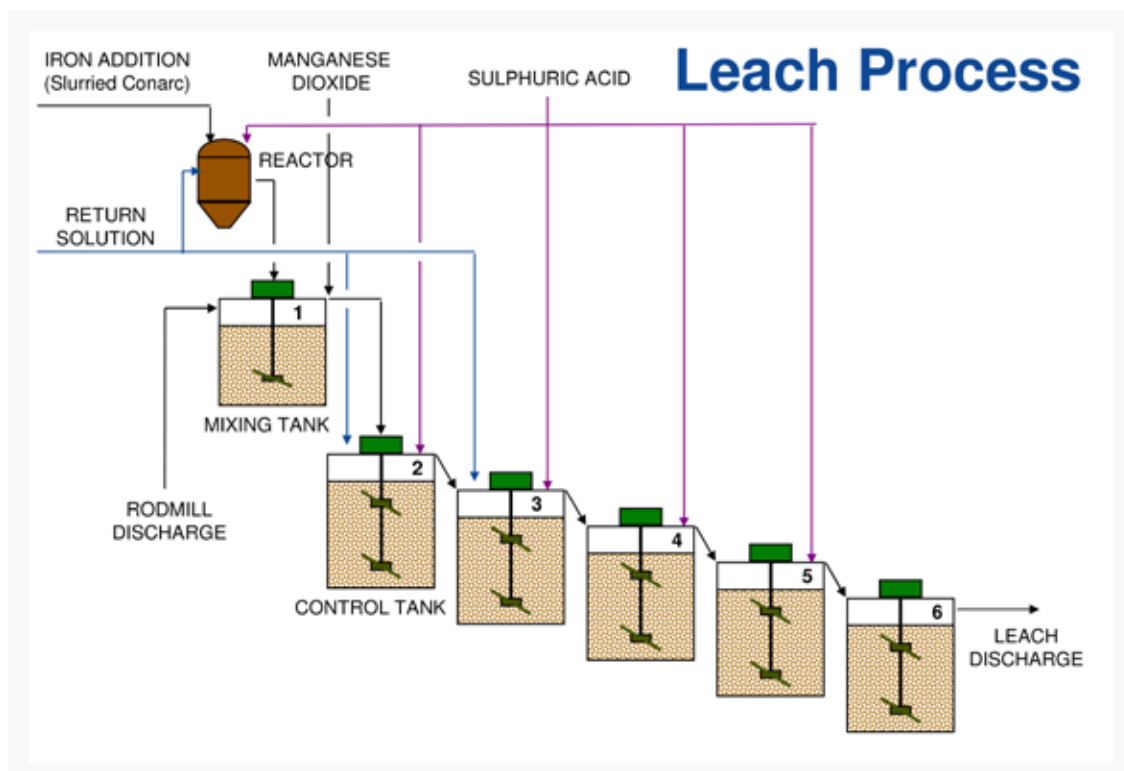
Figure 6: Leaching process
